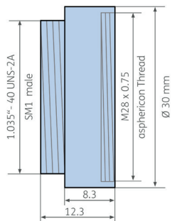
SM1 MALE
