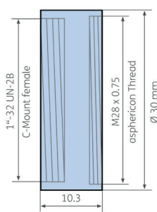
C-MOUNT FEMALE
