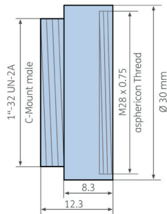
C-MOUNT MALE
