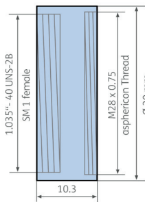
SM1 FEMALE
