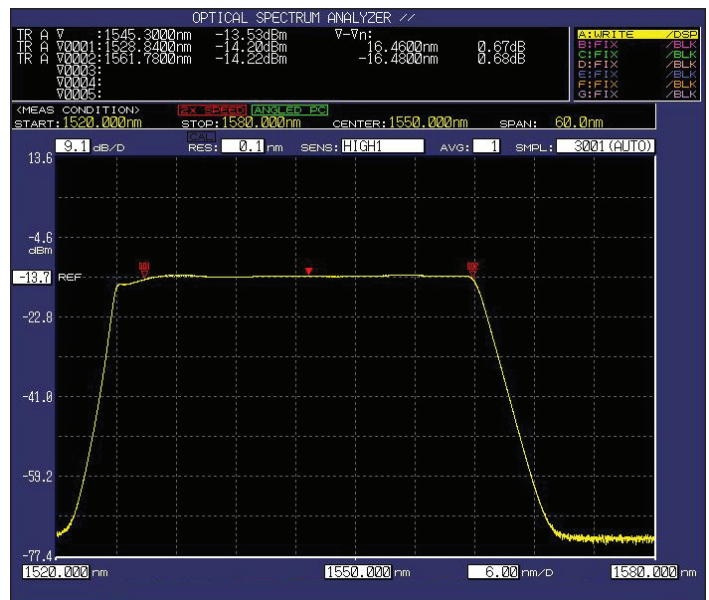
Figure 1. Output spectrum
